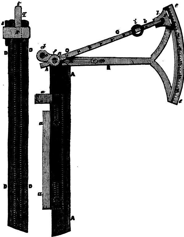
Fig. 223. Daniell's Pyrometer. No. 1 is the register. DDDD is the blacklead bar with its cavity, oo . At pppp it is cut away to the depth of half the bore. gg is the porcelain index, which is placed upon the top of the metallic bar, and confined to its place by the pressure of the platinum strap r , so acting by the force of the small porcelain wedge s . No. 2 represents the scale. AA is the principal brass rule, upon the under side of which the frame aaaaaa is adjusted by the screws bb , and which supports upon its bent extremity c , the arm B moving upon the centre d , and terminating in the arc of the circle ee . oc is the lighter arm moving upon the centre f upon the arm B , and carrying at one end the nonius g , and at the other the steel point h , the distance of which from the centre f is exactly half-an-inch, or one tenth of the radius fg , and equal to the distance of the two centres fd . x is a small lens, represented as lying down, but which may be raised by the centres k and l perpendicularly above the nonius to facilitate the reading. mm is the steel spring, which, being fixed in a cavity cut out of the arm B , presses upon a small pin n on the arm C , and throws the radius back to the commencement of the arc.
